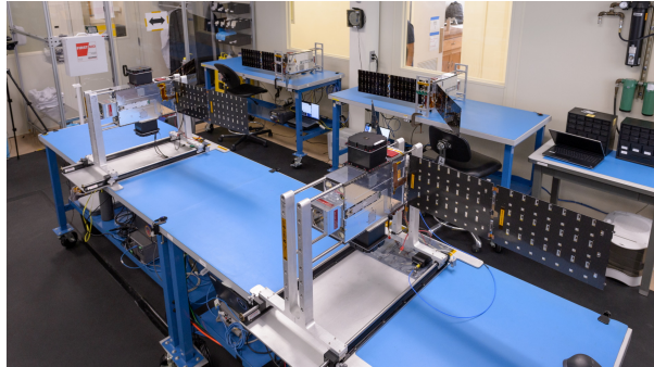
Figure 10: The four Starling CubeSats during integration. Credit: NASA/Dominic Hart (2022).
