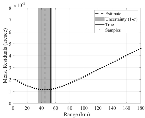
Figure 17: Initial target range estimation errors and uncertainties from BOD.
