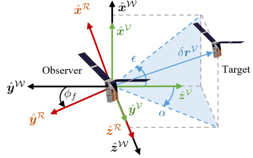
Figure 2: Definition of coordinate frames and bearing angles with VBS pointing in the -\hat{y}^{\mathcal{W}} direction.
